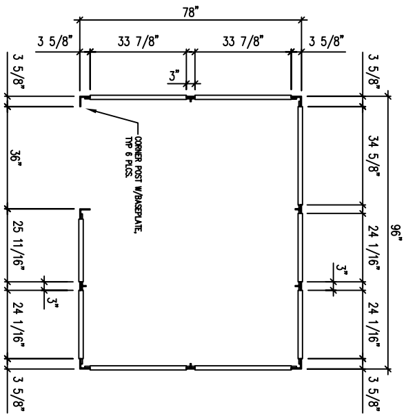
STYLE 'A' FLOOR PLAN
