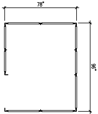
STYLE 'B' FLOOR PLAN
